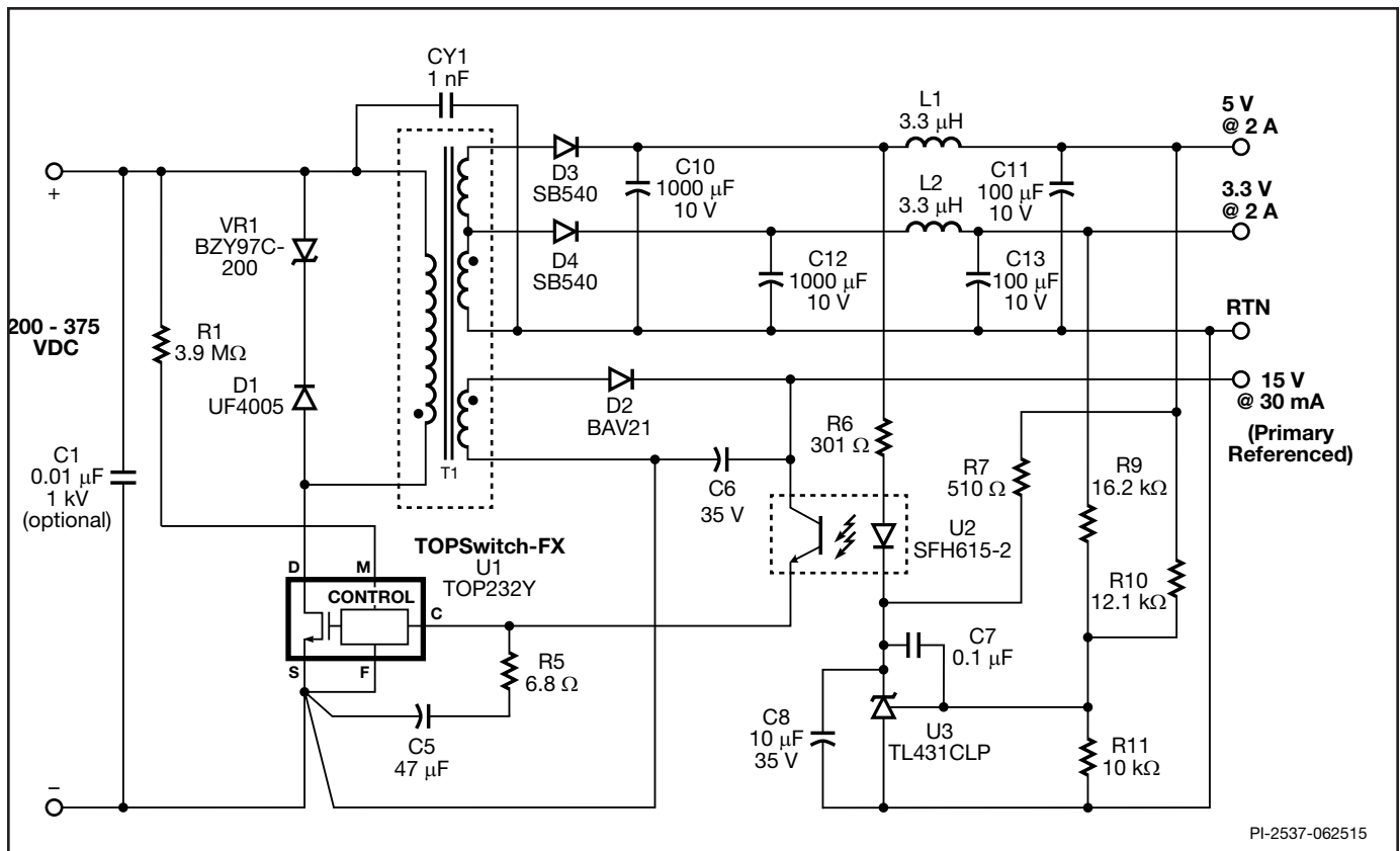
Figure 26. 17 W PC Standby Supply.
